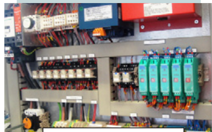
100kw bespoke soft start drive panel for oil and gas site. This panel also consists of IS circuits for field devices.
